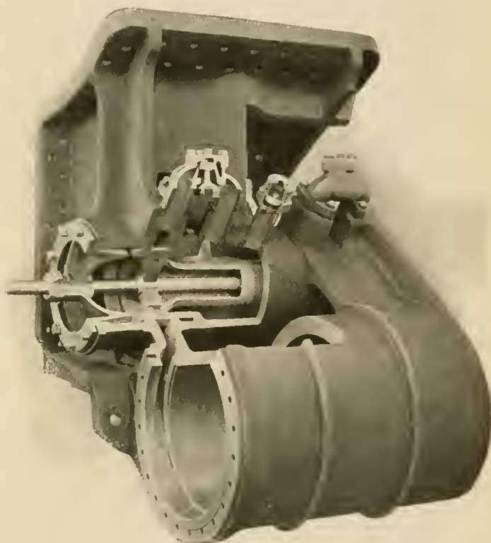
FIG. 2.—PISTON VALVE AND BY-PASS VALVES.
